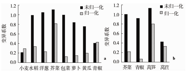
图 5 归一化前后各物种铜 (a) 和镍 (b) 的 EC_{10} 的种内变异 Fig. 5 Intra-species variability of EC_{10} values of copper (a) and nickel (b) to various species before and after normalizaition
