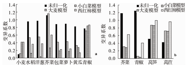
图 3 归一化前后各物种铜 (a) 和镍 (b) 的 EC_{50} 的种内变异, Fig. 3 Intra-species variability of EC_{50} values of copper (a) and nickel (b) to various species before and after normalizaition
